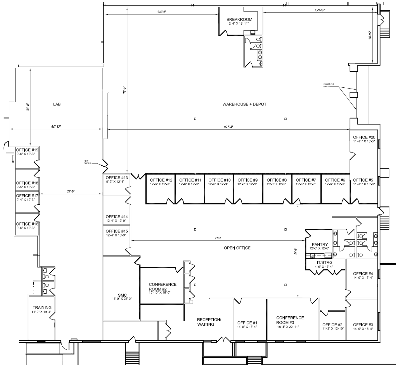
1 PROPOSED PLAN SCALE: NTS
