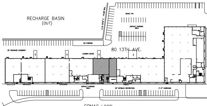
3 LOCATION PLAN SCALE: NTS
