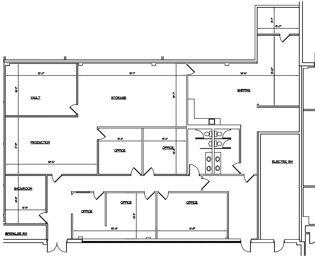
1 EXISTING PLAN SCALE: NTS
