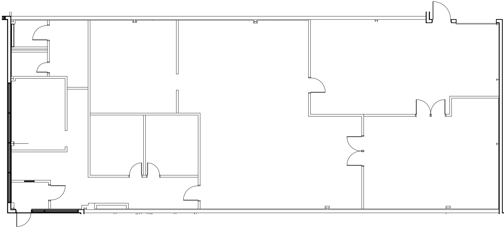
1 EXISTING PLAN SCALE: NTS
