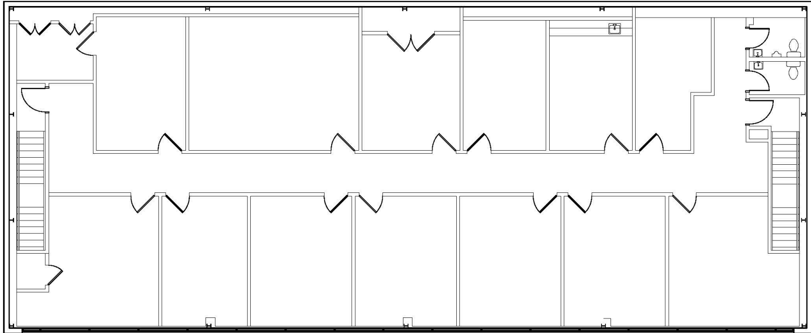
1 EXISTING PLAN SCALE: NTS
