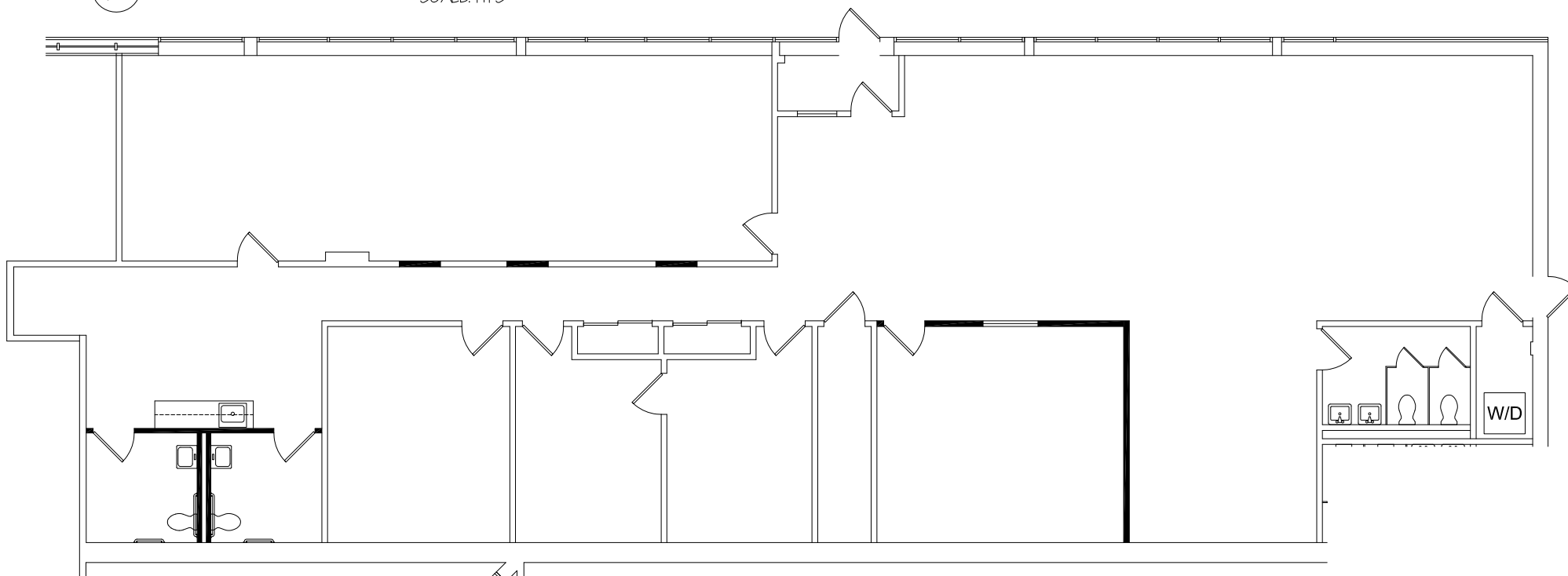
PROPOSED PLAN
